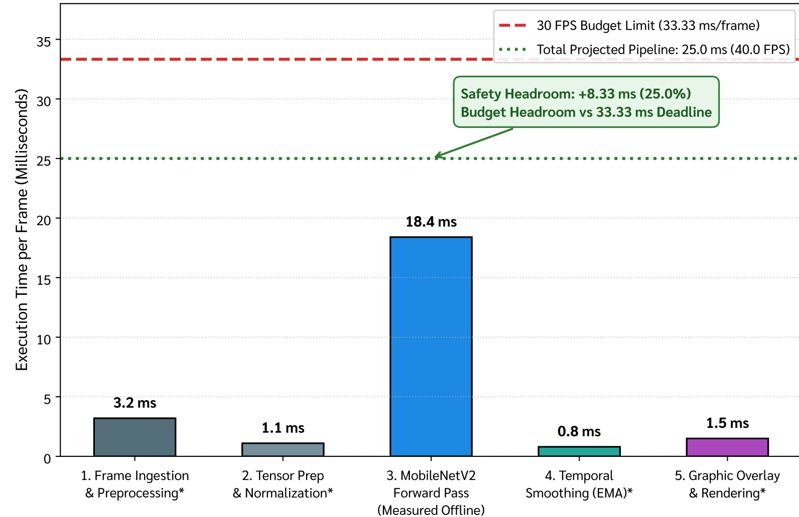
Figure 7(b): Architectural Latency Budget Simulation (*Simulated Allowances; 18.4 ms Measured on Apple Silicon arm64)
