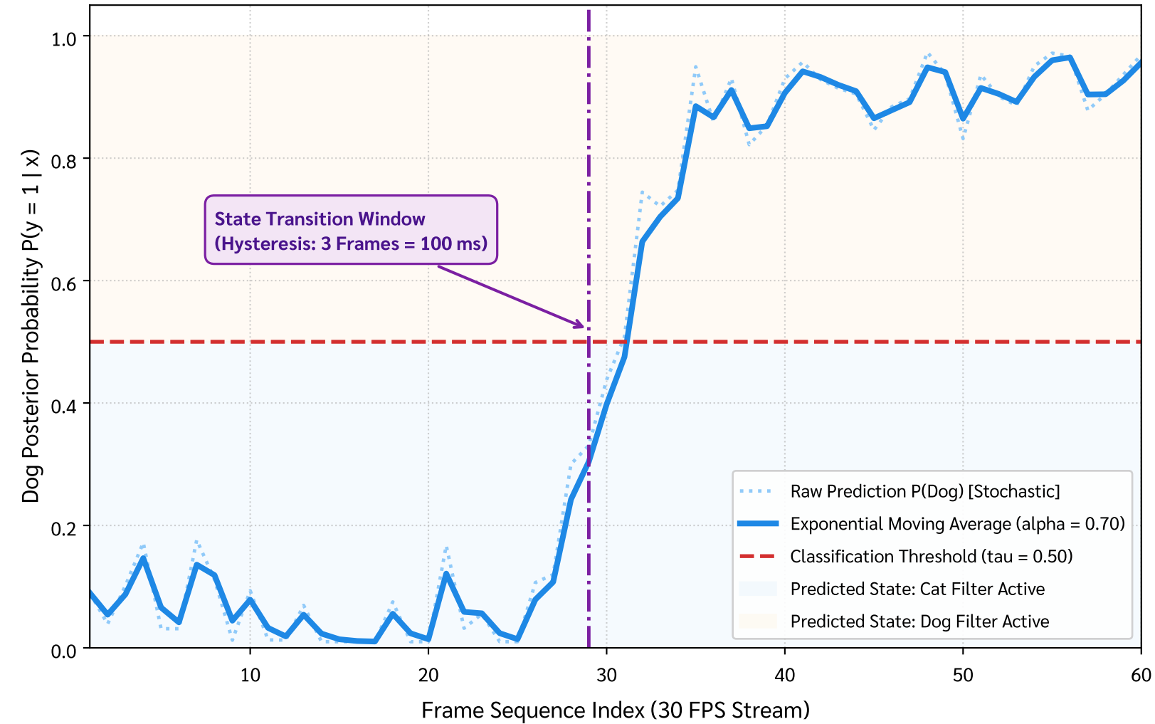
Figure 7(a): Simulated 60-Frame Streaming Timeline (Temporal Exponential Smoothing: \alpha = 0.70 )
